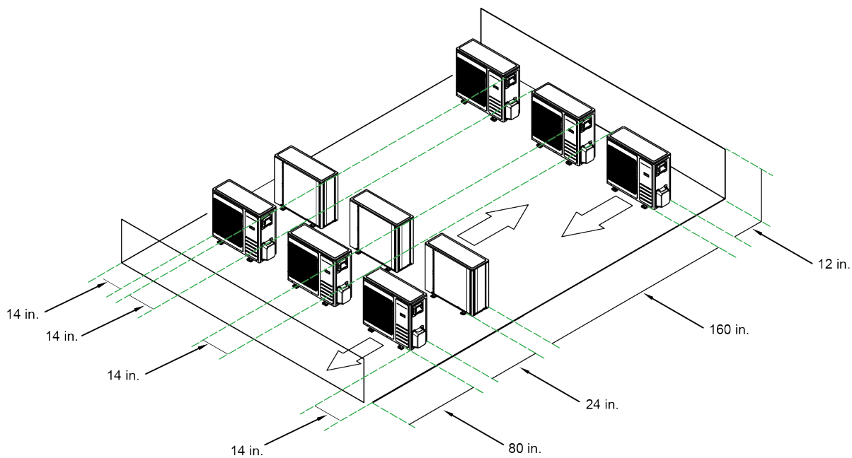
Figure 5: Alternative installation clearances for multiple units
